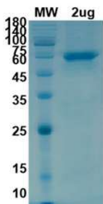
Final sample QC. Coomassie blue staining
